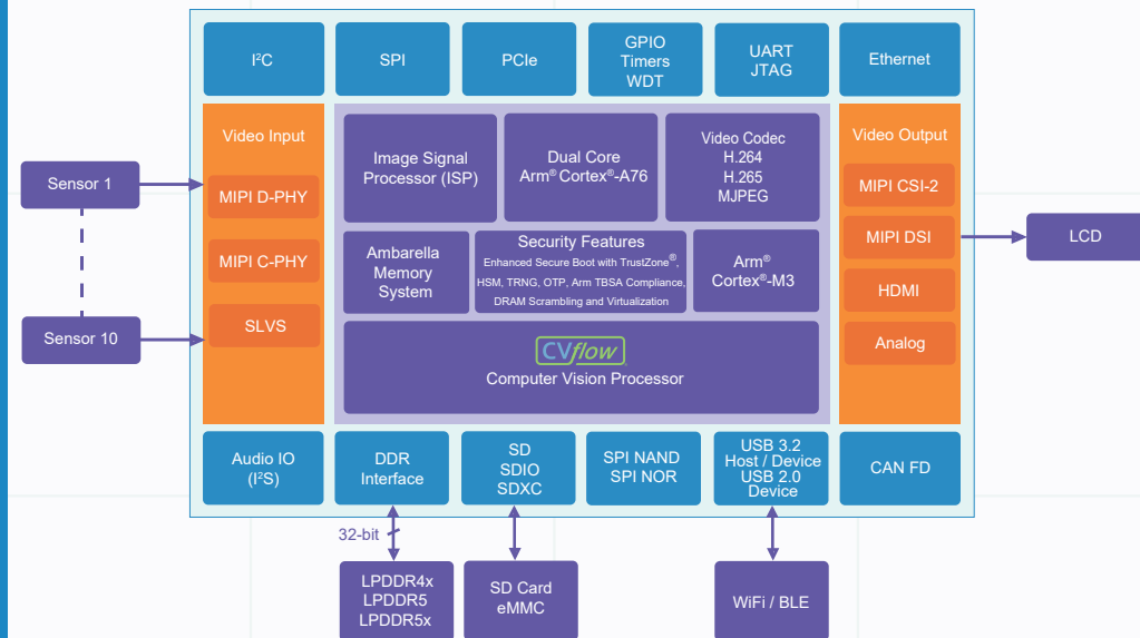
CV72S Block Diagram
