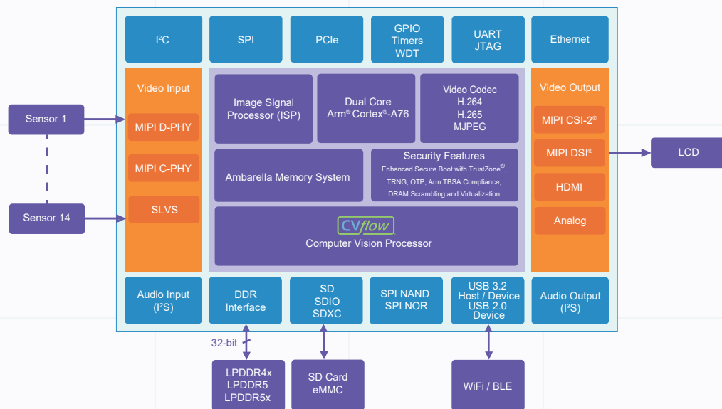
CV52 Block Diagram
